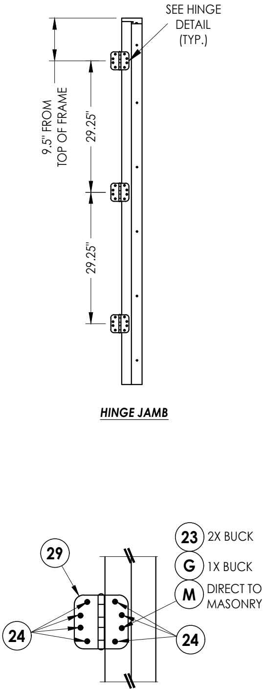
HINGE DETAIL
