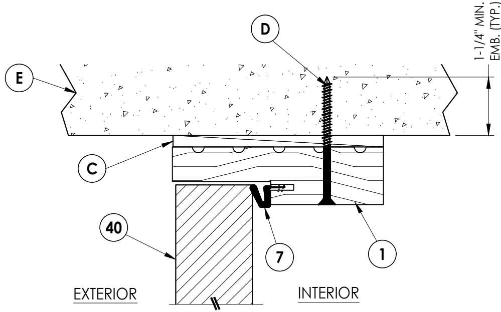
3 6 VERTICAL CROSS SECTION Shown Direct to Masonry Outswing only
